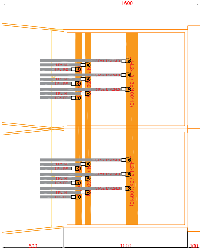
FRONT PANEL VIEW
