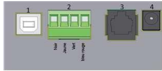
Connectors
