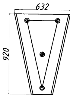
BOTTOM LINER 2 PCS AYK 621
