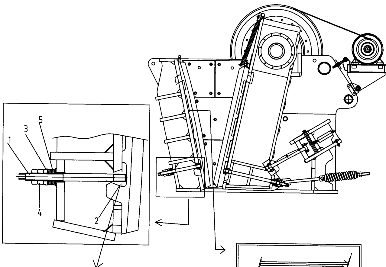
FIXED JAW WEDGE (NO: 2)
