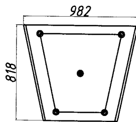
MIDDLE LINER 2 PCS AYK 623
