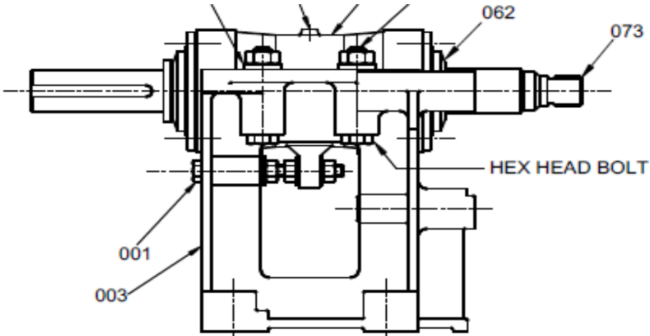
Fig. 1 Frame Assembly
