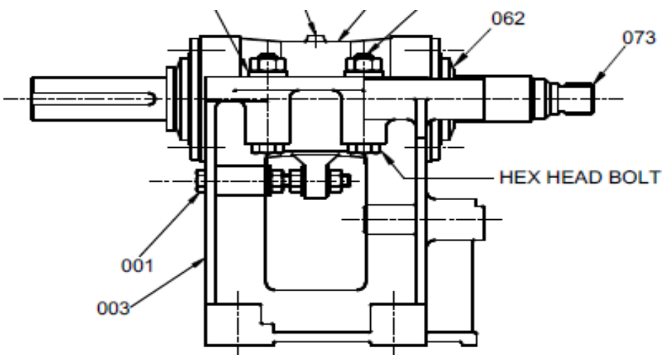
Fig. 1 Frame Assembly
