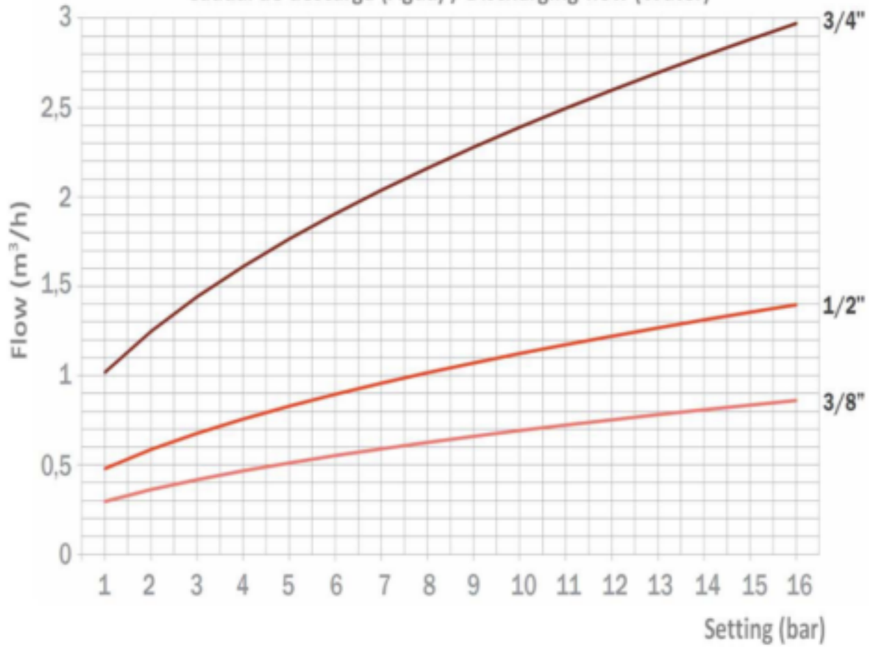
Caudal de descarga (Agua) / Discharging flow (Water)
